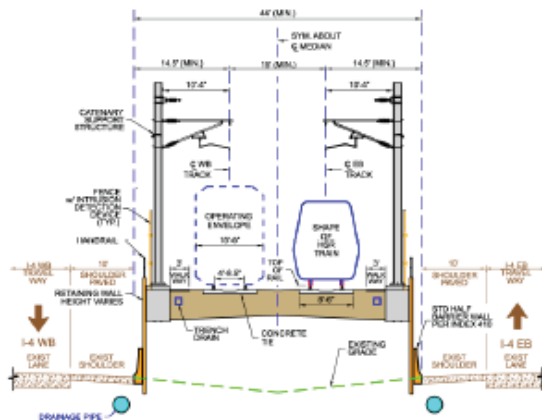
RETAINING WALL SECTION
