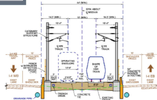
TIGHT SECTION IN I-4 MEDIAN
