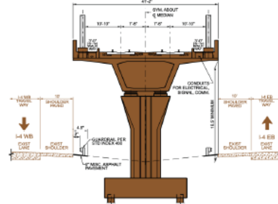
VIADUCT
