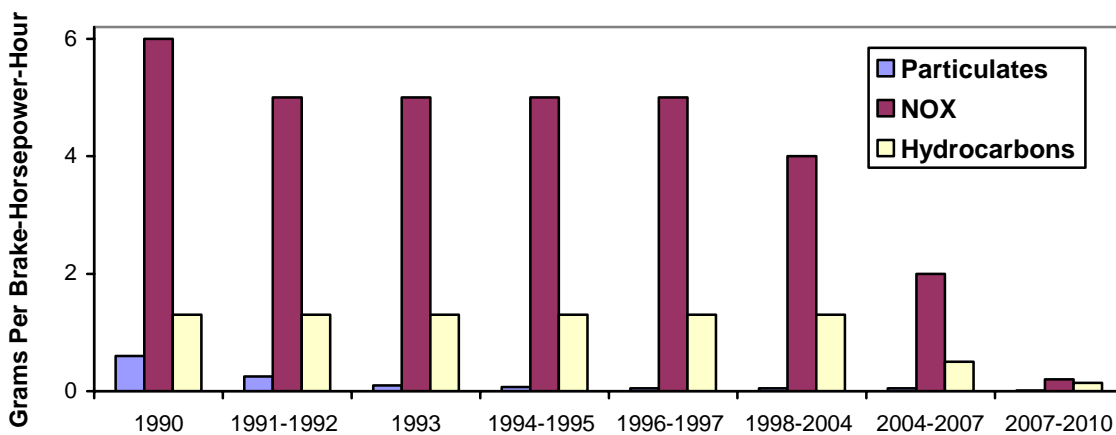
Figure 9 Federal Transit Bus Emissions Standards (USDOT 2006, Table 3)
