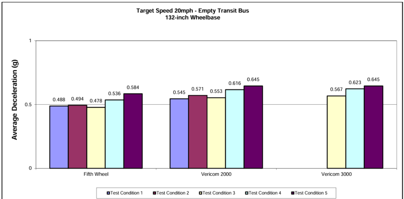
FIGURE 3 Short Wheelbase Transit Bus
