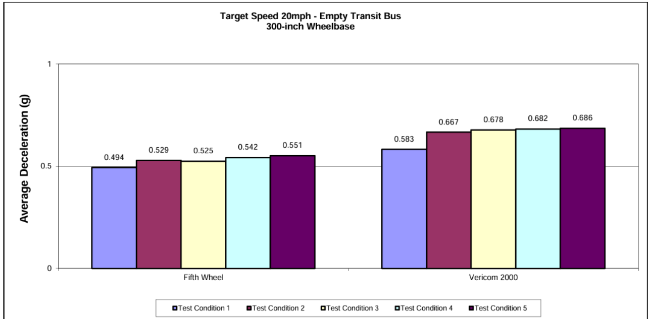
FIGURE 1 Long Wheelbase Transit Bus
