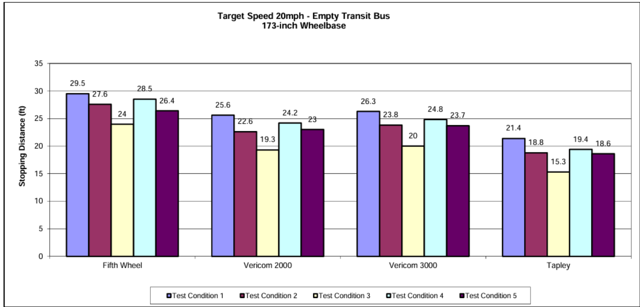
FIGURE 2 Medium Wheelbase Transit Bus
