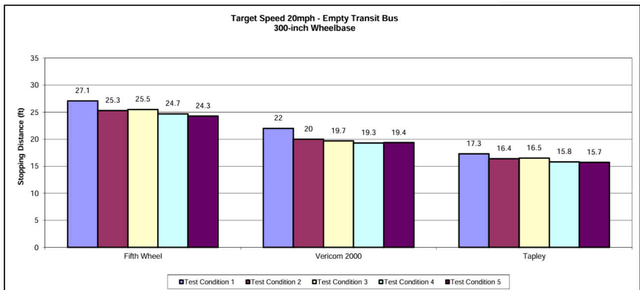
FIGURE 1 Long Wheelbase Transit Bus
