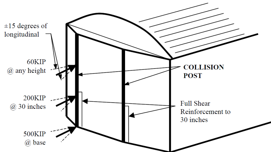
FIGURE 2 Schematic of Collision Post Loads for the Cab End of Cab Cars
