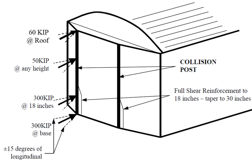
FIGURE 3 Schematic of Collision Post Loads for Coach Cars
