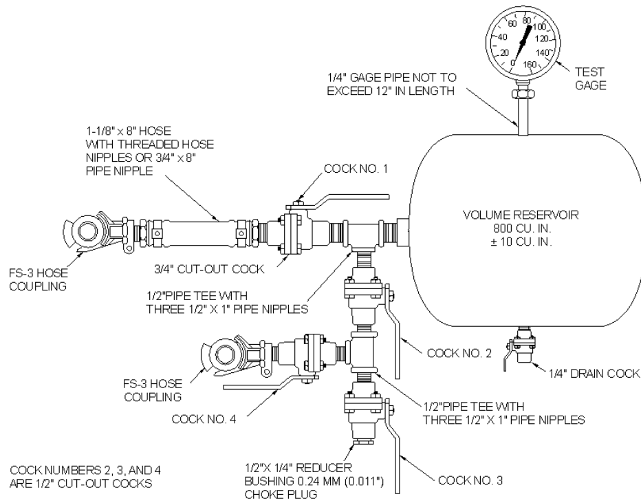
FIGURE 7 Alternate Rack for Testing the Passenger Single Car Testing Device
