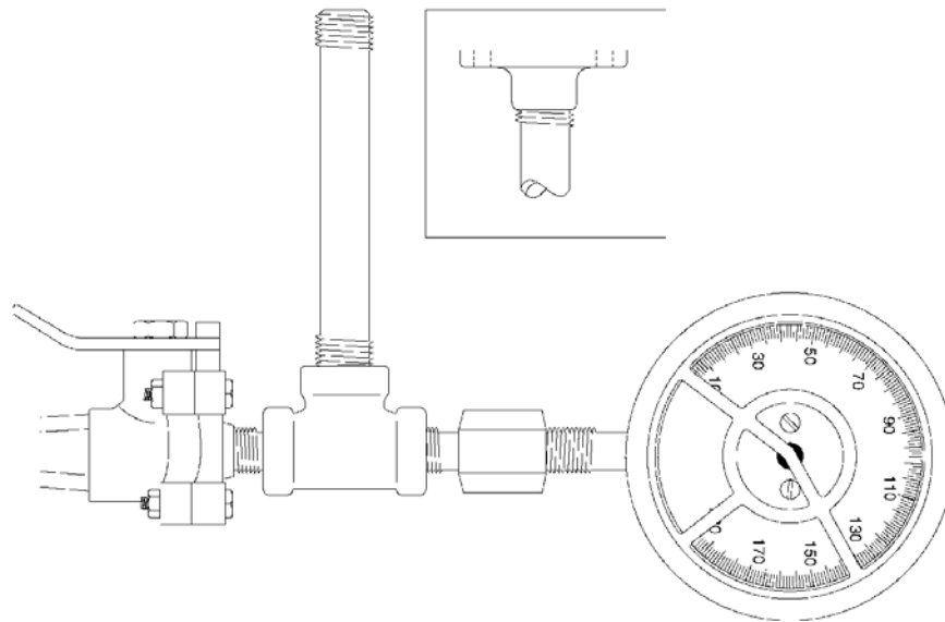
FIGURE 4 Test Gauge: Bleed Cock Arrangement
