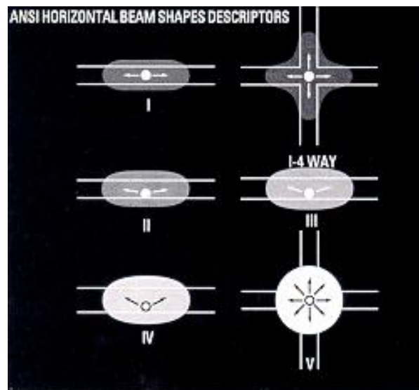
FIGURE 1 ANSI Horizontal Beam Shapes Descriptors
