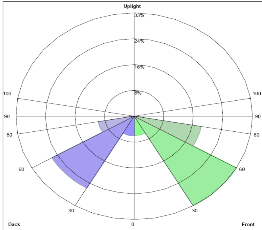
LUMINAIRE CLASSIFICATION SYSTEM (LCS) GRAPH
